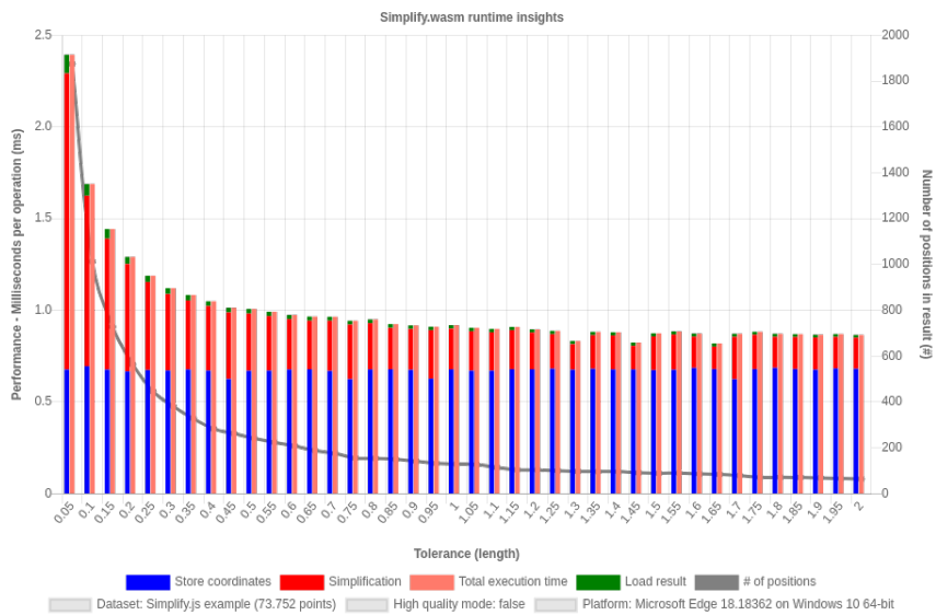
Figure 10: Simplify.wasm runtime analysis benchmark result of Windows device with Edge browser on dataset "Simplify.js example" without high Quality mode.
