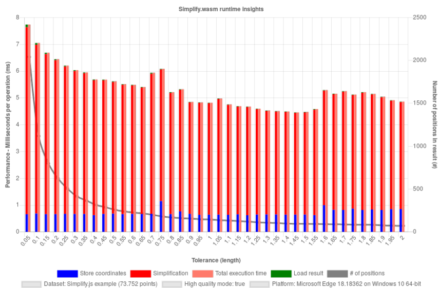
Figure 19: Simplify.wasm runtime analysis benchmark result of Windows device with Edge browser on dataset "Simplify.js example" with high quality mode.
