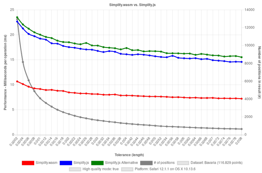
Figure 22: Simplify.wasm vs. Simplify.js benchmark result of MacBook Pro device with Safari browser on dataset "Bavaria outline" with high quality mode.
