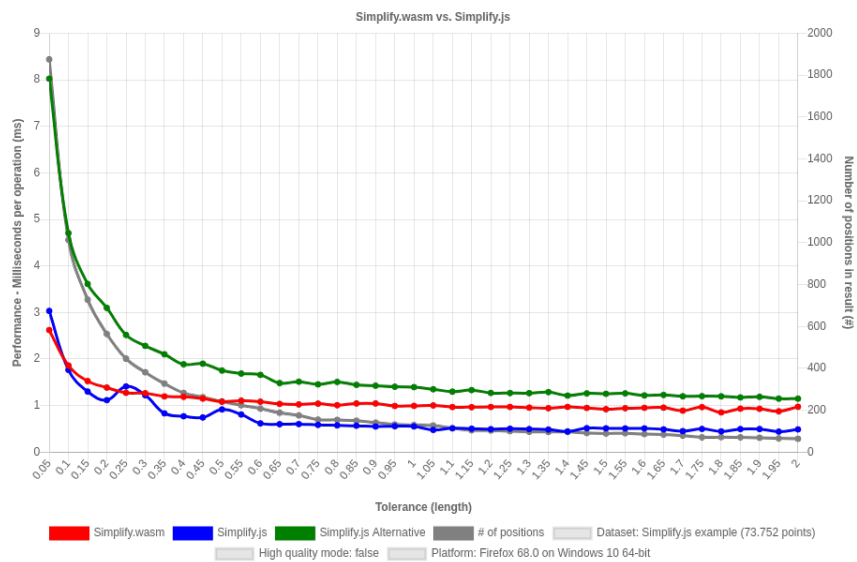
Figure 13: Simplify.wasm vs. Simplify.js benchmark result of Windows device with Firefox browser on dataset "Simplify.js example" without high quality mode.
