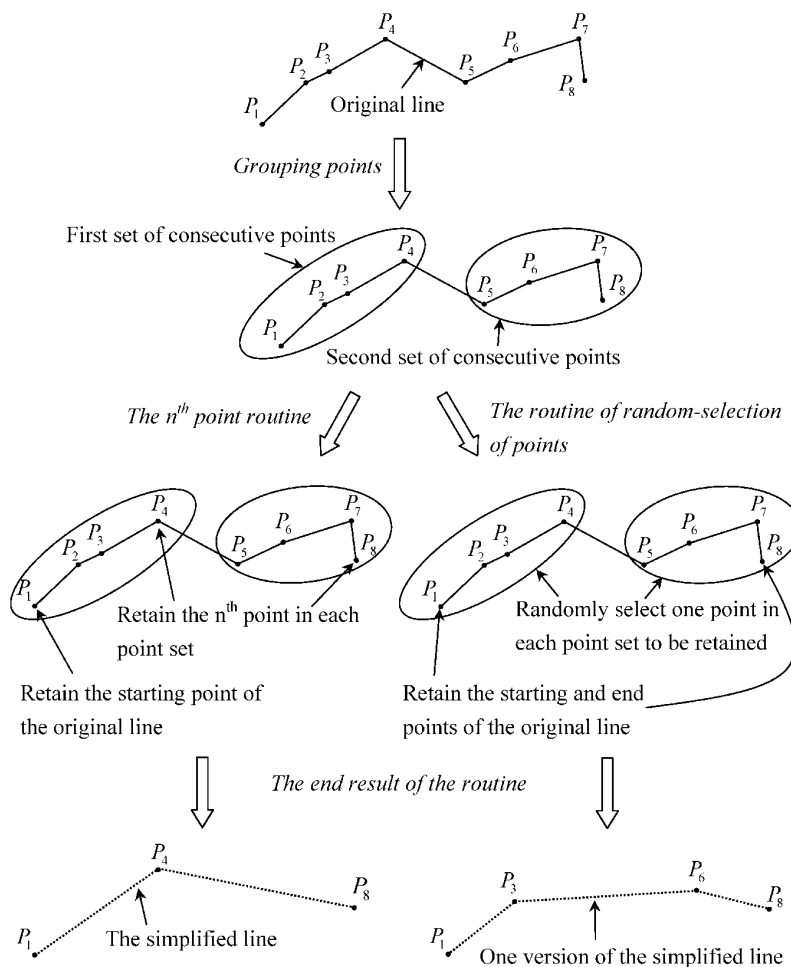
Figure 1: Nth point algorithm
