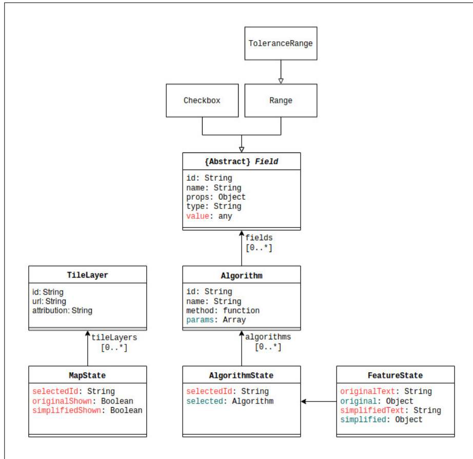
Figure 10: The state model of the application
