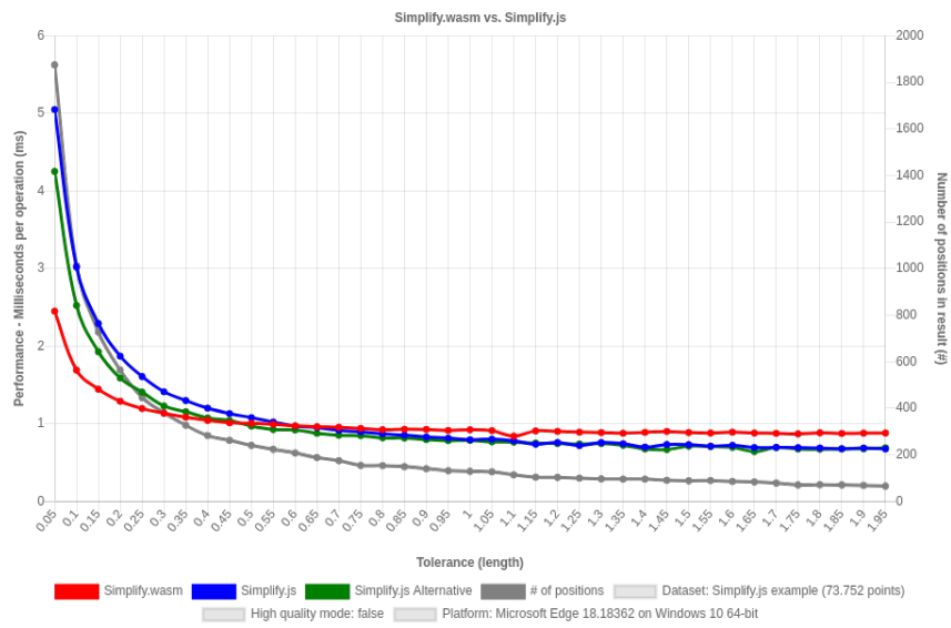
Figure 14: Simplify.wasm vs. Simplify.js benchmark result of Windows device with Edge browser on dataset "Simplify.js example" without high quality mode.
