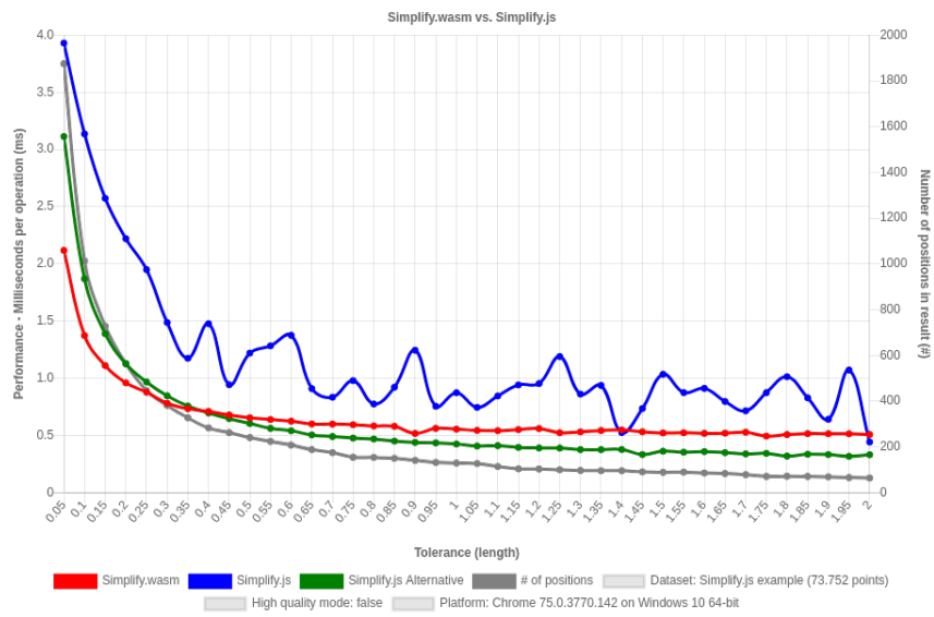
Figure 12: Simplify.wasm vs. Simplify.js benchmark result of Windows device with Chrome browser on dataset "Simplify.js example" without high quality mode.
