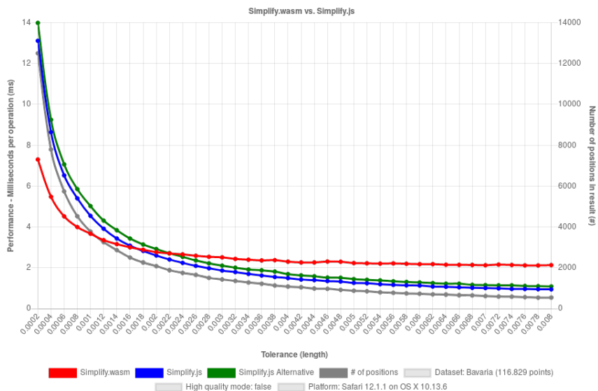
Figure 20: Simplify.wasm vs. Simplify.js benchmark result of MacBook Pro device with Safari browser on dataset "Bavaria outline" without high quality mode.
