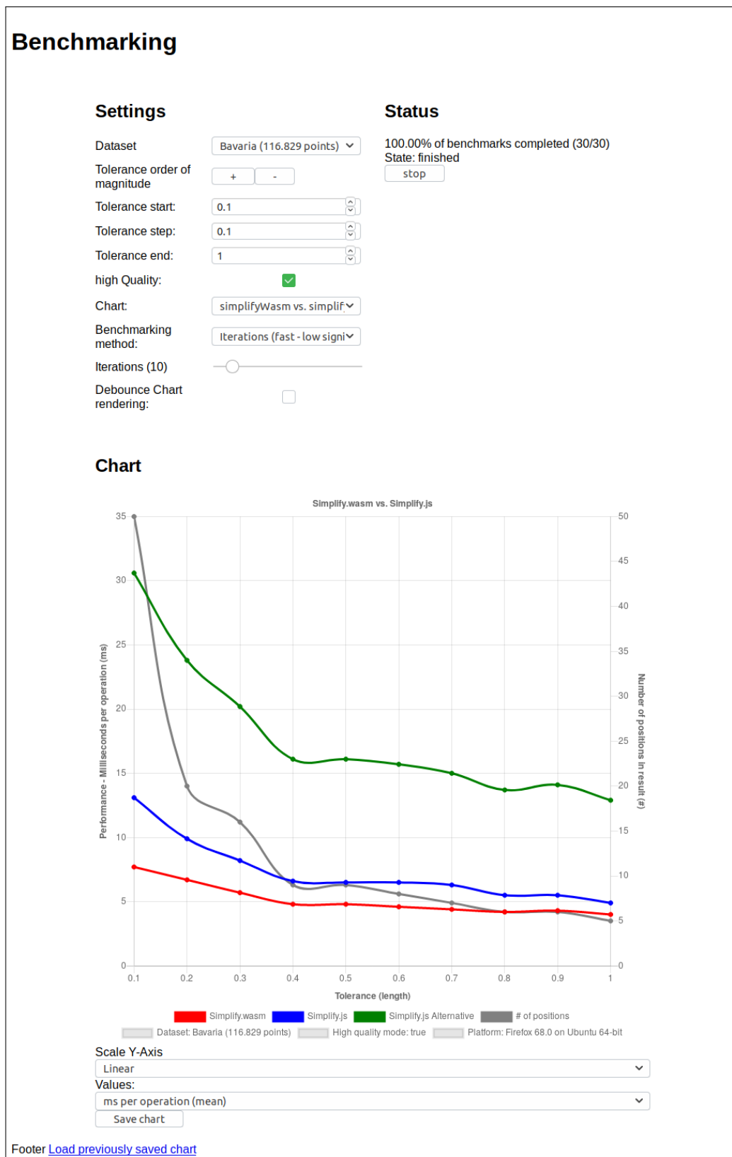
Figure 9: The user interface for benchmarking application. (not final)
