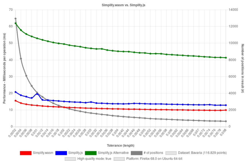
Figure 26: Simplify.wasm vs. Simplify.js benchmark result of Ubuntu device with Firefox browser on dataset "Bavaria outline" with high quality mode.
