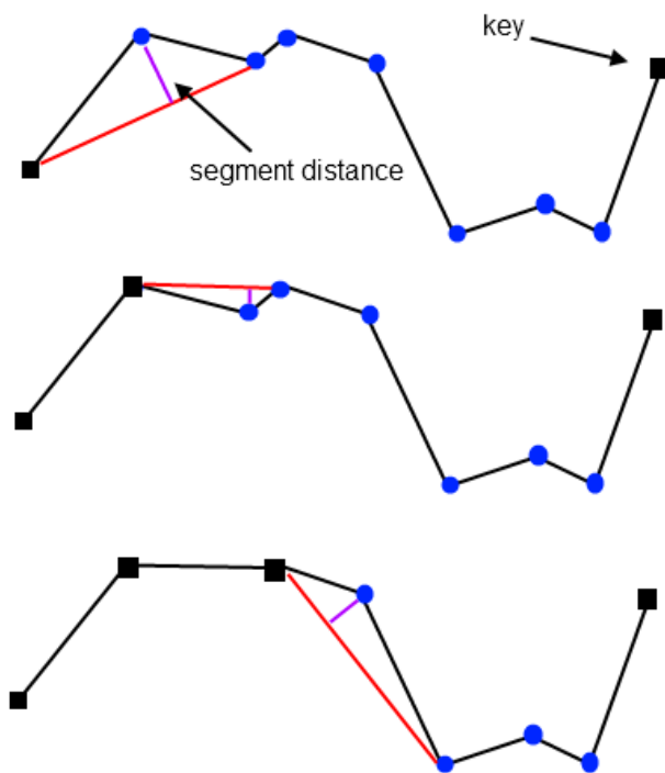
Figure 3: Perpendicular distance algorithm
