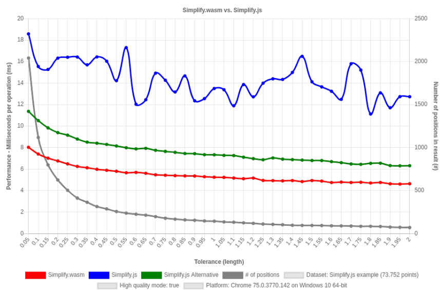
Figure 15: Simplify.wasm vs. Simplify.js benchmark result of Windows device with Chrome browser on dataset "Simplify.js example" with high quality mode.
