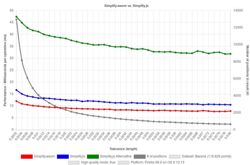
Figure 23: Simplify.wasm vs. Simplify.js benchmark result of MacBook Pro device with Firefox browser on dataset "Bavaria outline" with high quality mode.
