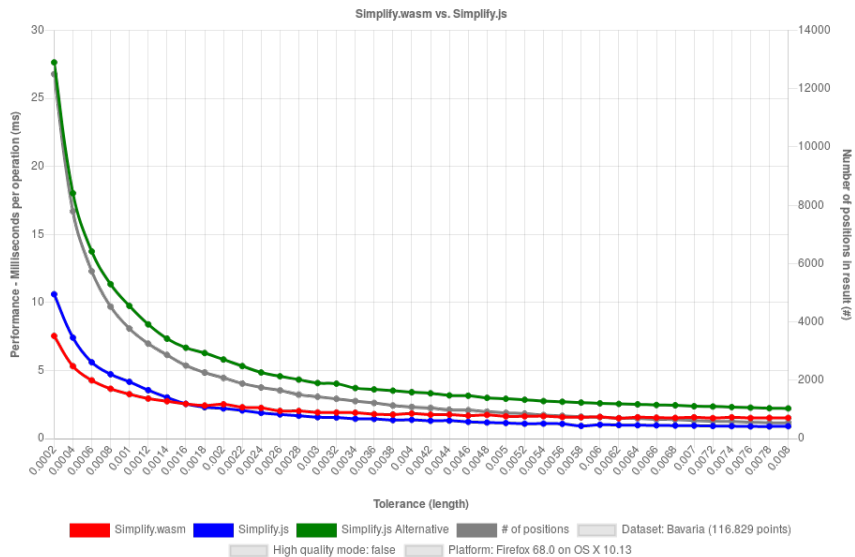
Figure 21: Simplify.wasm vs. Simplify.js benchmark result of MacBook Pro device with Firefox browser on dataset "Bavaria outline" without high quality mode.
