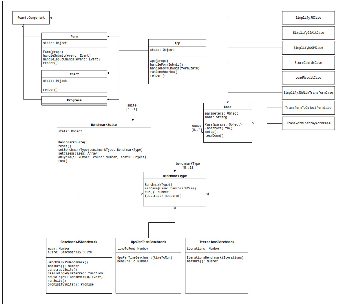
Figure 8: UML diagram of the benchmarking application
