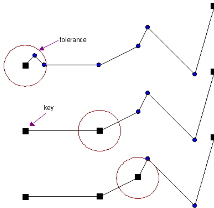
Figure 2: Radial distance algorithm
