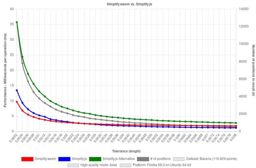
Figure 24: Simplify.wasm vs. Simplify.js benchmark result of Ubuntu device with Firefox browser on dataset "Bavaria outline" without high quality mode.
