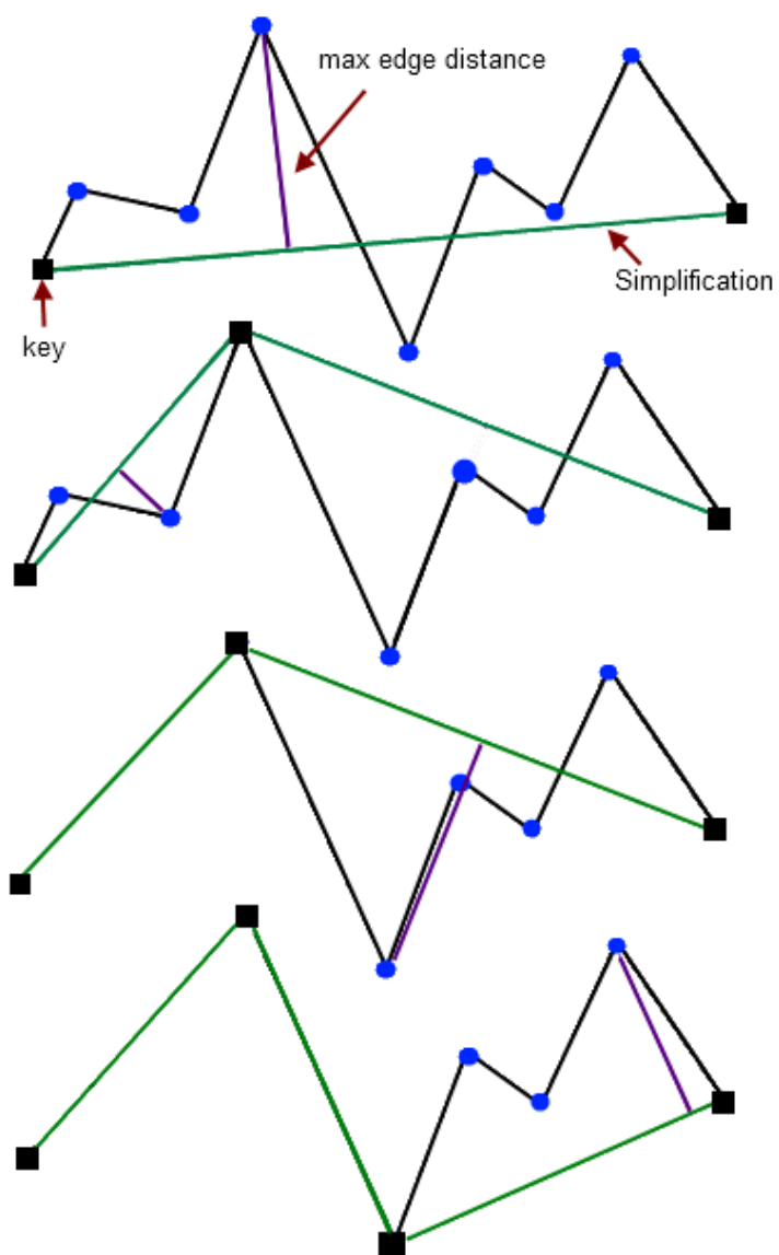
Figure 7: Douglas Peucker algorithm
