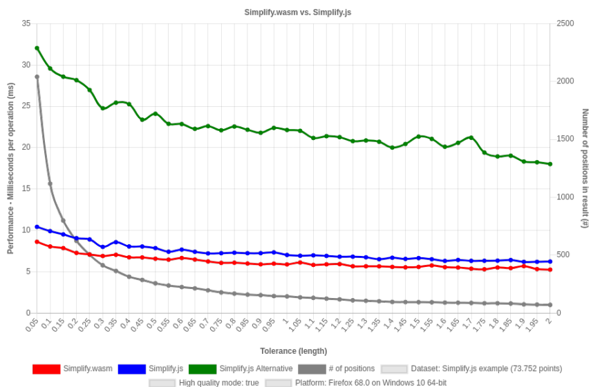
Figure 16: Simplify.wasm vs. Simplify.js benchmark result of Windows device with Firefox browser on dataset "Simplify.js example" with high quality mode.
