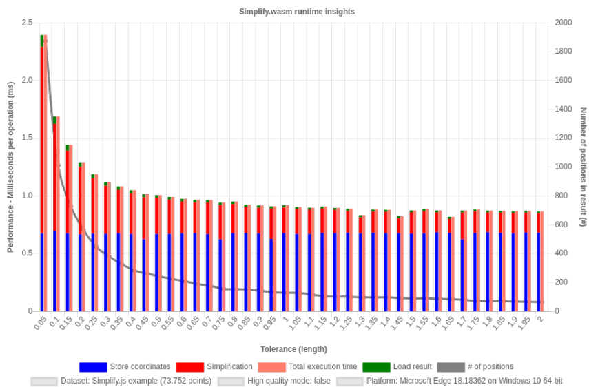
Figure 18: Simplify.wasm runtime analysis benchmark result of Windows device with Edge browser on dataset "Simplify.js example" without high quality mode.
