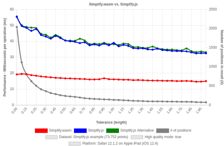
Figure 25: Simplify.wasm vs. Simplify.js benchmark result of iPad device with Safari browser on dataset "Simplify.js example" with high quality mode.
