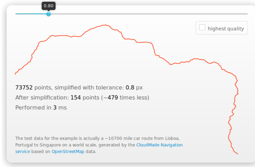
Figure 6: The Simplify.js test data visualized
