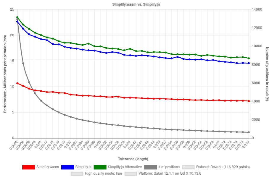
Figure 16: Simplify.wasm vs. Simplify.js benchmark result of MacBook Pro device with Safari browser on dataset "Bavaria outline" with high quality mode.
