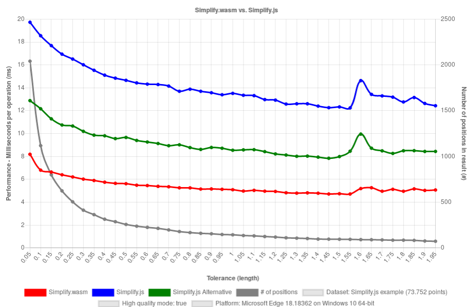
Figure 11: Simplify.wasm vs. Simplify.js benchmark result of Windows device with Edge browser on dataset "Simplify.js example" with high quality mode.
