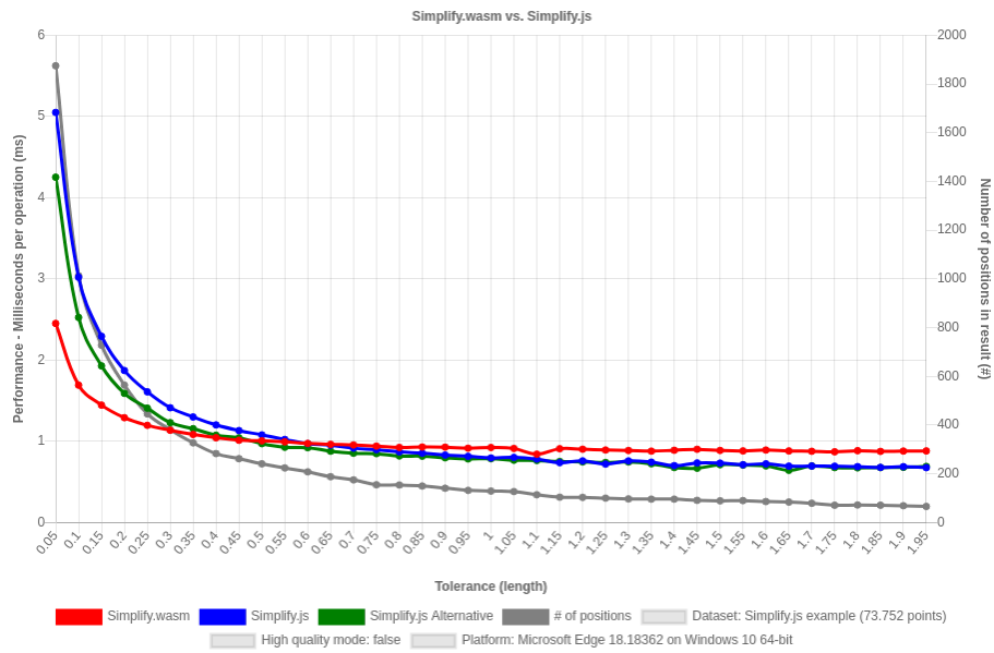
Figure 8: Simplify.wasm vs. Simplify.js benchmark result of Windows device with Edge browser on dataset "Simplify.js example" without high quality mode.
