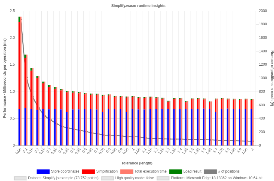
Figure 12: Simplify.wasm runtime analysis benchmark result of Windows device with Edge browser on dataset "Simplify.js example" without high quality mode.
