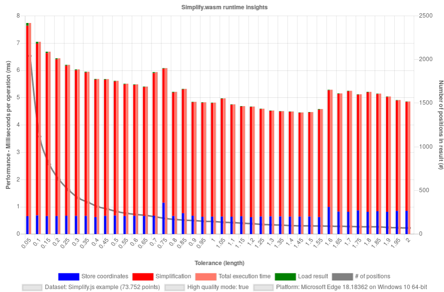
Figure 13: Simplify.wasm runtime analysis benchmark result of Windows device with Edge browser on dataset "Simplify.js example" with high quality mode.
