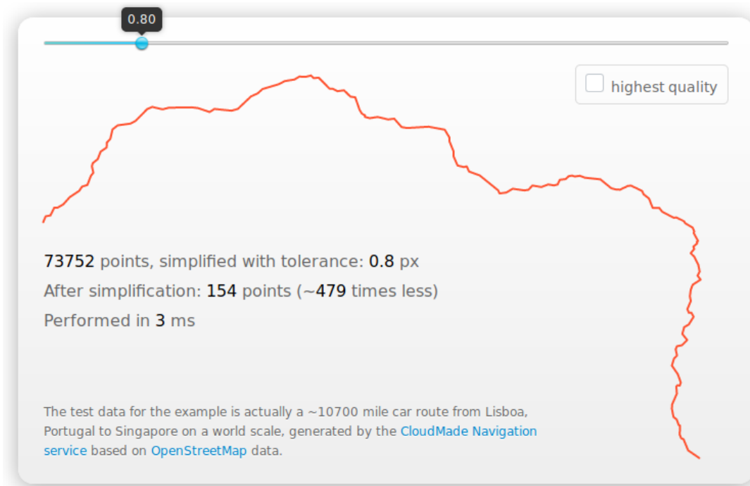
Figure 4: The Simplify.js test data visualized
