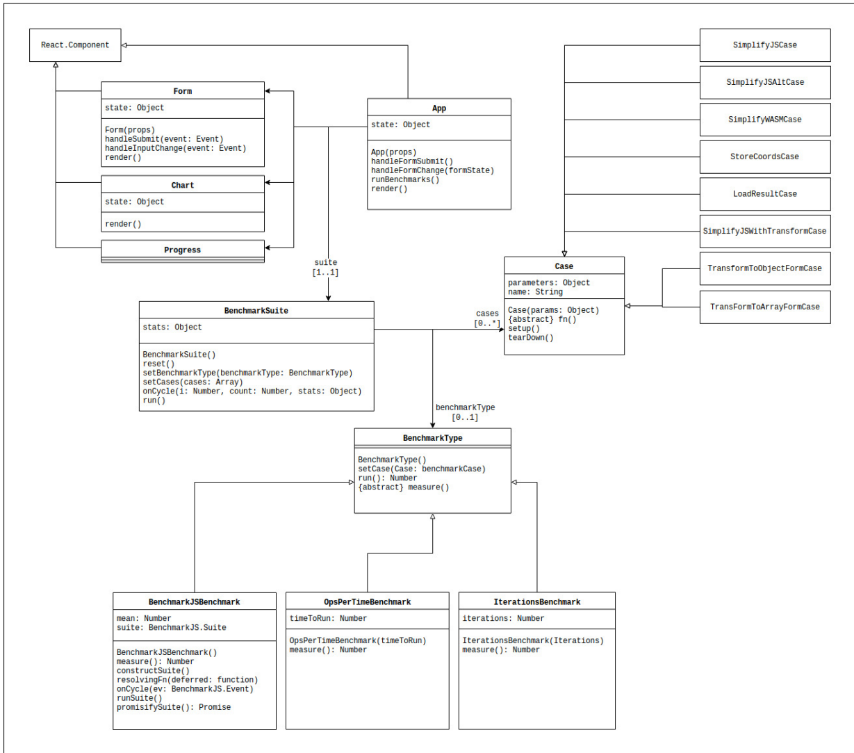
Figure 1: UML diagram of the benchmarking application
