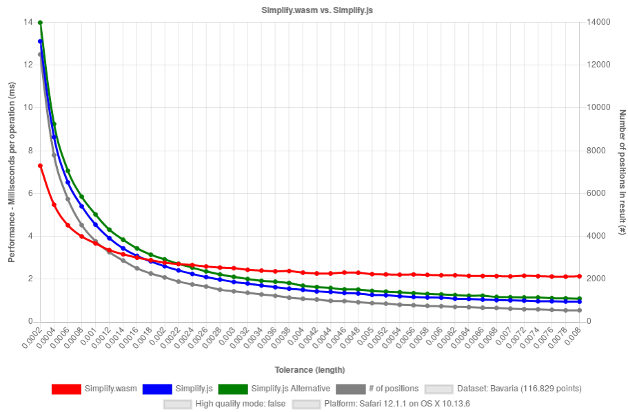
Figure 14: Simplify.wasm vs. Simplify.js benchmark result of MacBook Pro device with Safari browser on dataset "Bavaria outline" without high quality mode.
