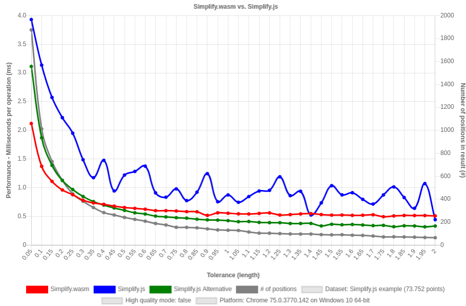
Figure 6: Simplify.wasm vs. Simplify.js benchmark result of Windows device with Chrome browser on dataset "Simplify.js example" without high quality mode.
