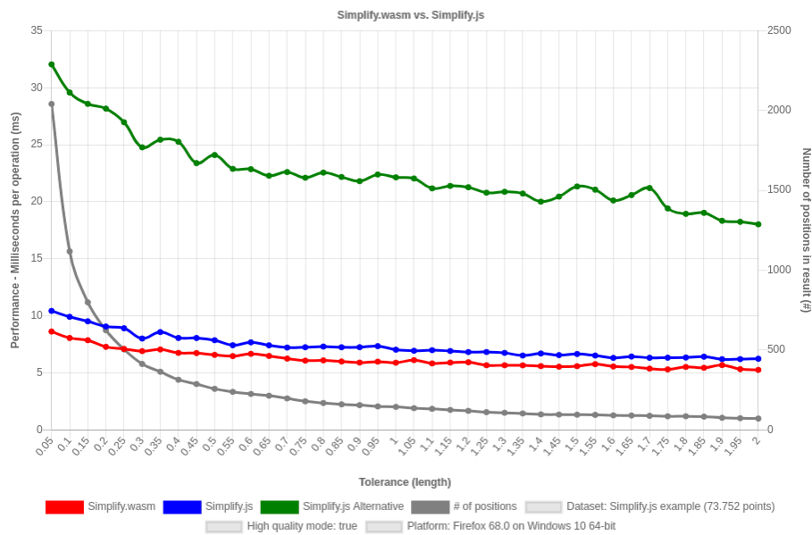
Figure 10: Simplify.wasm vs. Simplify.js benchmark result of Windows device with Firefox browser on dataset "Simplify.js example" with high quality mode.
