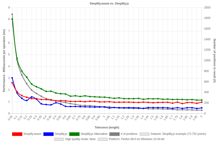
Figure 7: Simplify.wasm vs. Simplify.js benchmark result of Windows device with Firefox browser on dataset "Simplify.js example" without high quality mode.
