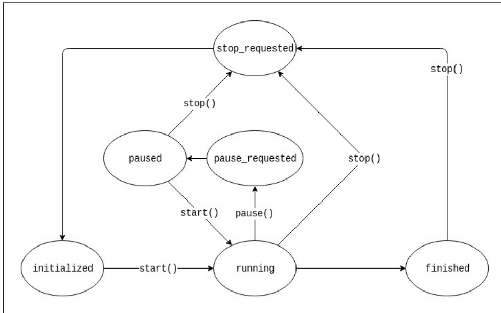
Figure 2: The state machine for the benchmark suite
