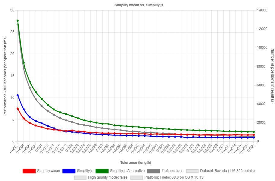
Figure 15: Simplify.wasm vs. Simplify.js benchmark result of MacBook Pro device with Firefox browser on dataset "Bavaria outline" without high quality mode.
