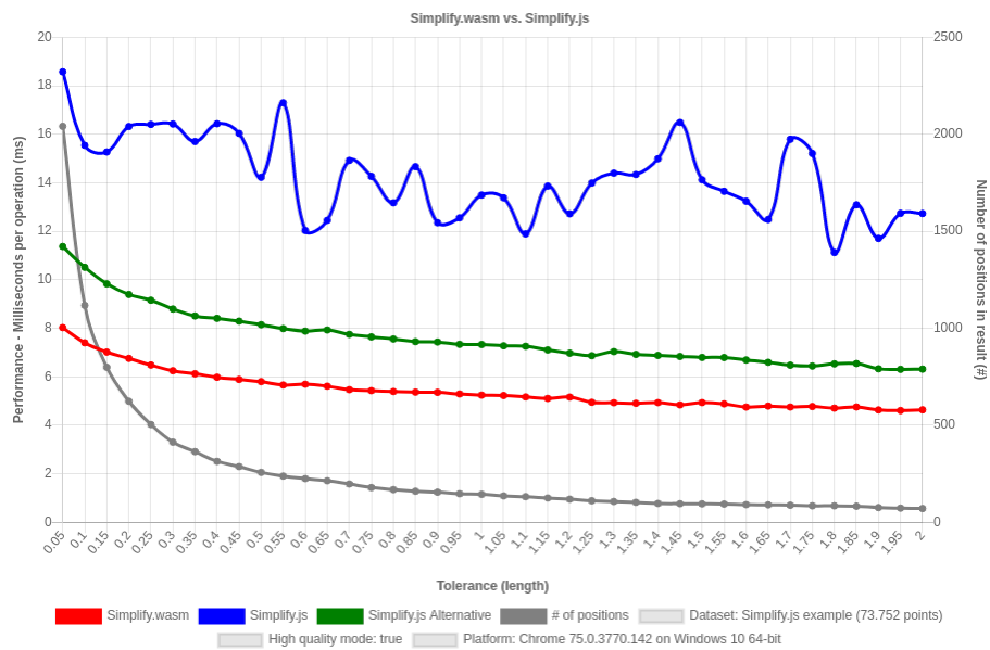
Figure 9: Simplify.wasm vs. Simplify.js benchmark result of Windows device with Chrome browser on dataset "Simplify.js example" with high quality mode.
