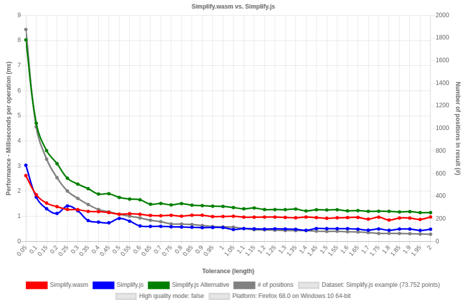
Figure 7: Simplify.wasm vs. Simplify.js benchmark result of Windows device with Firefox browser on dataset "Simplify.js example" without high quality mode.
