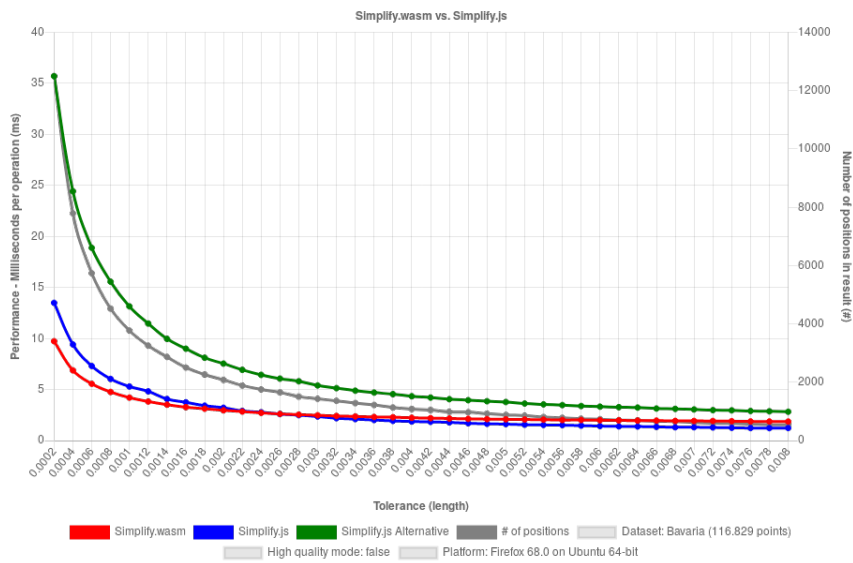
Figure 18: Simplify.wasm vs. Simplify.js benchmark result of Ubuntu device with Firefox browser on dataset "Bavaria outline" without high quality mode.
