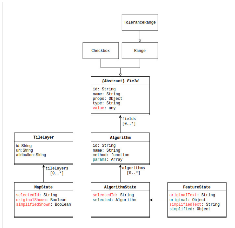
Figure 22: The state model of the application
