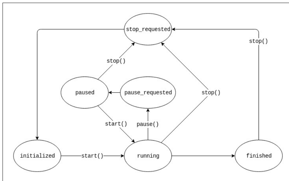
Figure 2: The state machine for the benchmark suite
